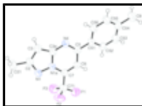
Fig. 1. View of the asymmetric unit of the title compound, showing the atom labelling scheme. Displacement ellipsoids are drawn at the 50% probability level. H atoms are represented by circles of arbitrary radii.
